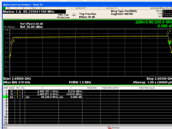
Hopping Sequence_2DH5
