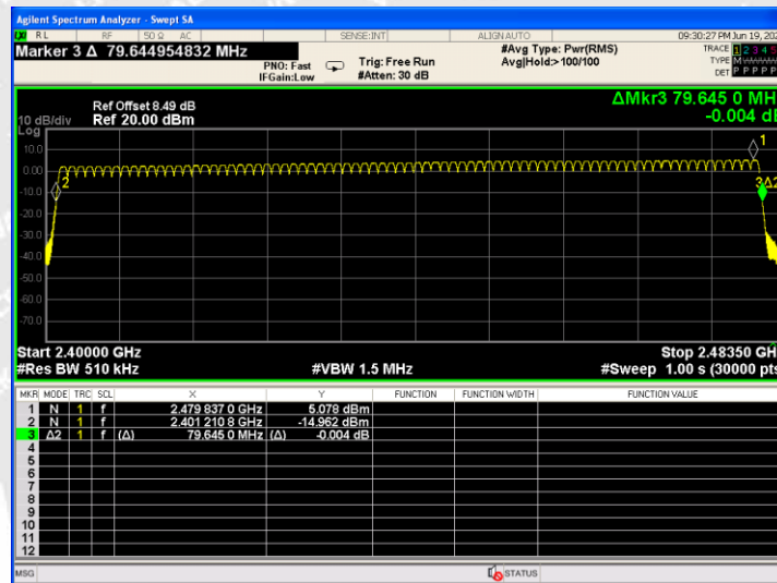
Hopping Sequence_DH5
