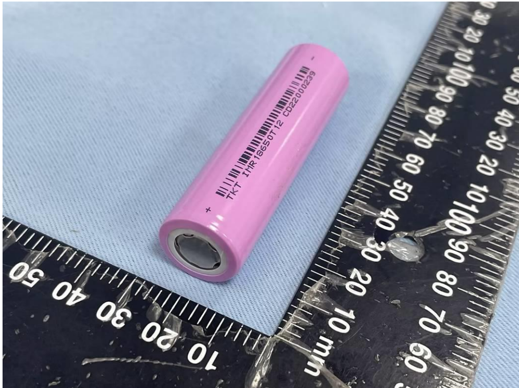
Picture 1 Top view of cell (Model: IMR18650T12)
