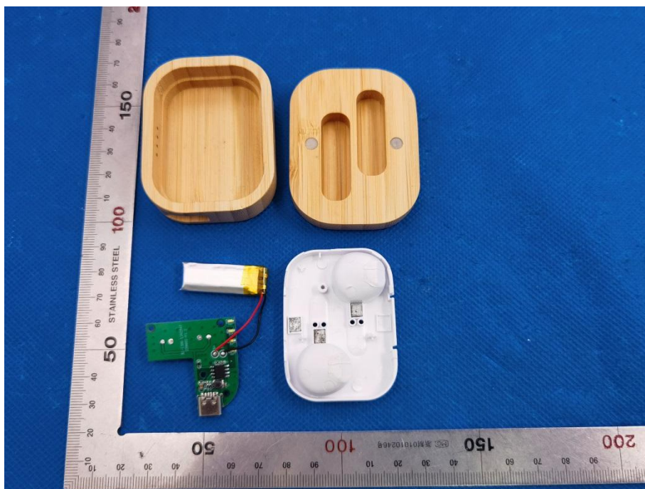
Fig.6 – open view (charging base)
