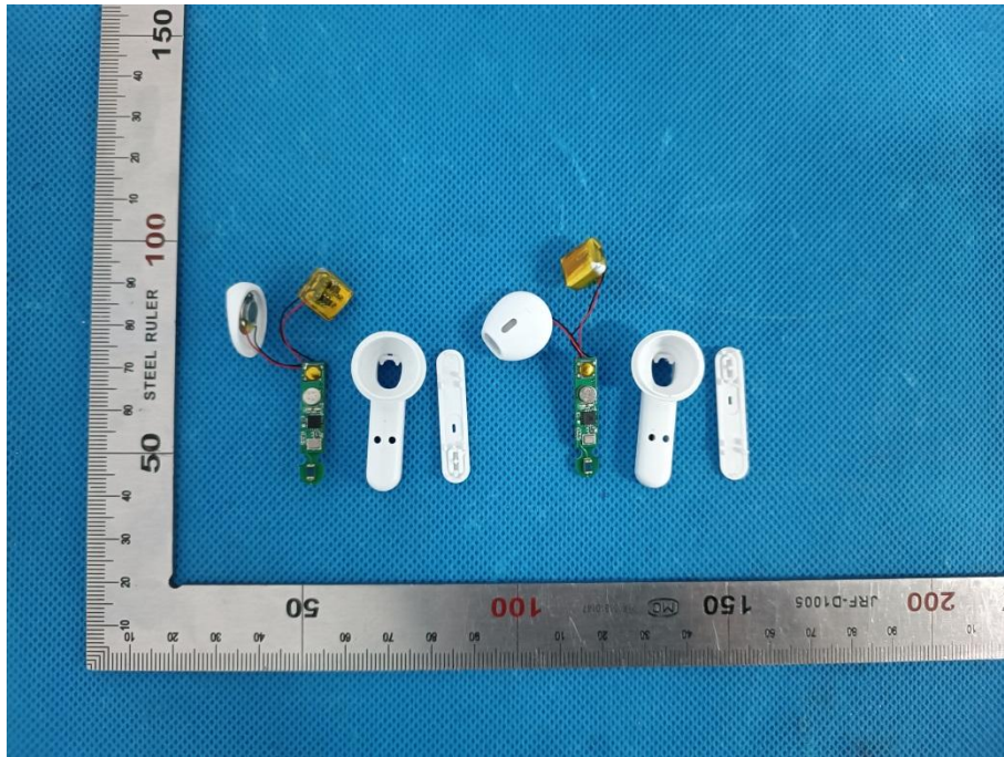
Fig.13 – open view (Earphone)
