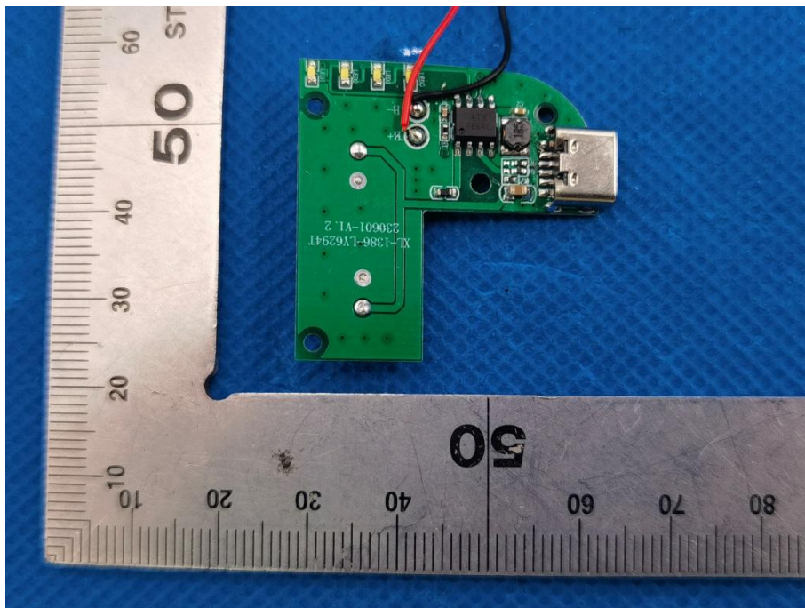
Fig.7 – PCB view (charging base)
