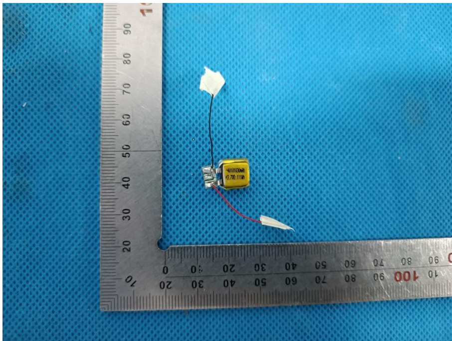
Fig.16 – battery view (Earphone)
