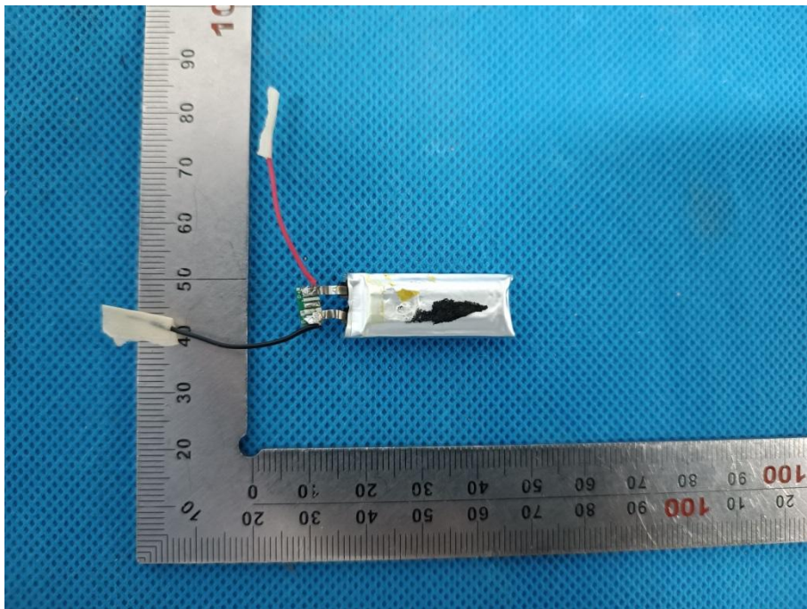
Fig.10 – battery view (charging base)
