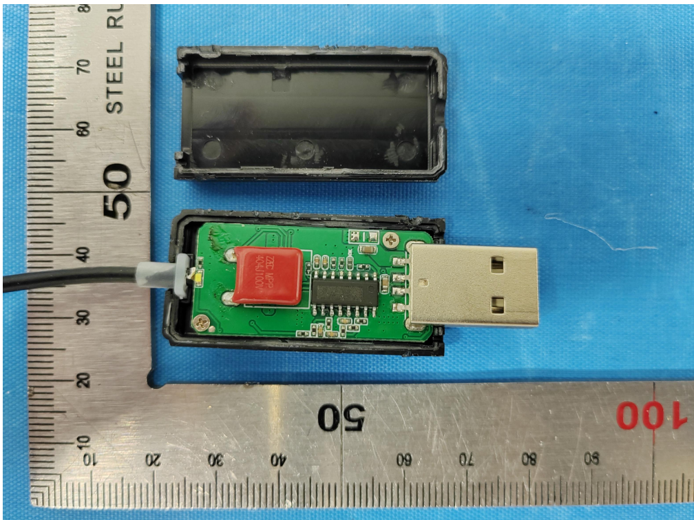
Fig.4 – Internal view
