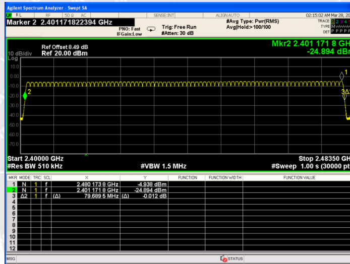
Hopping Sequence_DH5
