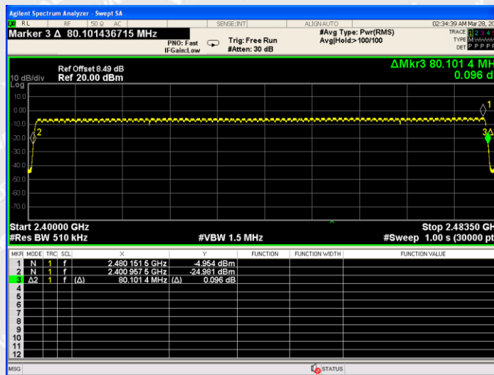
Hopping Sequence_2DH5
