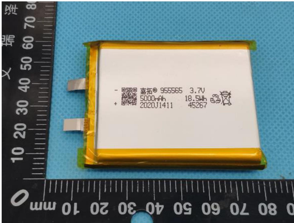
Fig. 9 – Battery view
