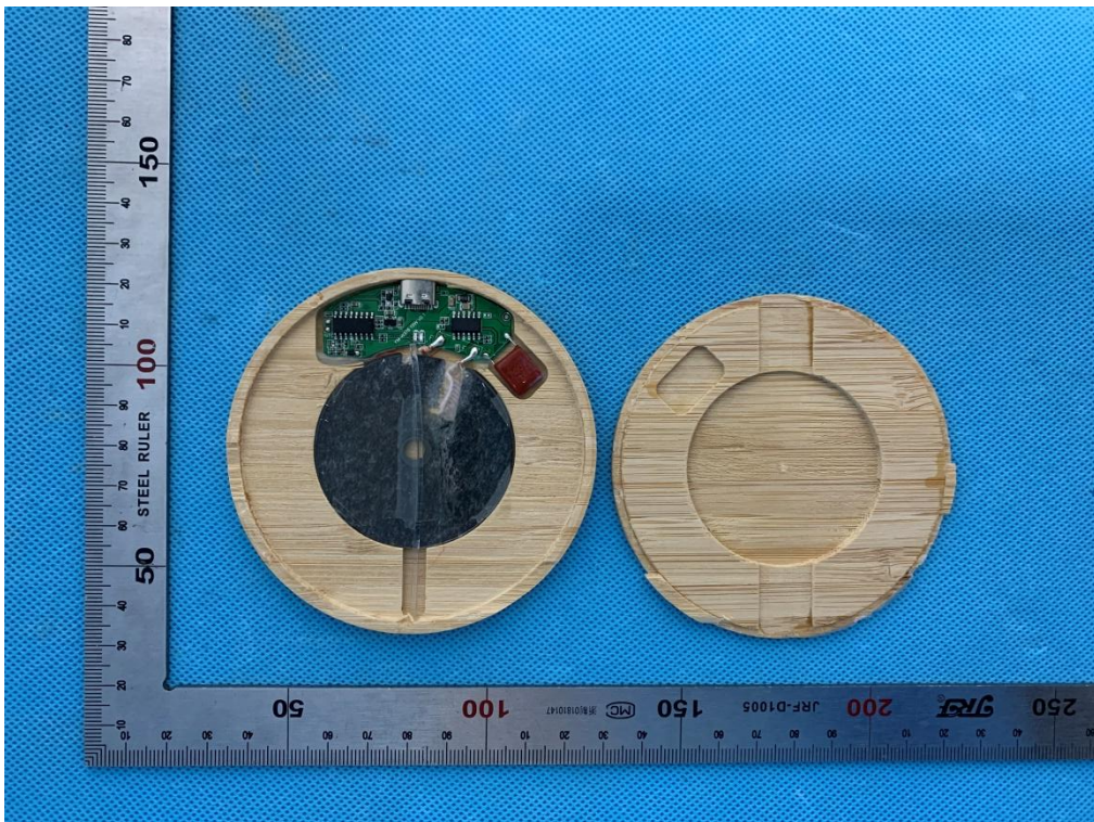
Figure 4 Open view
