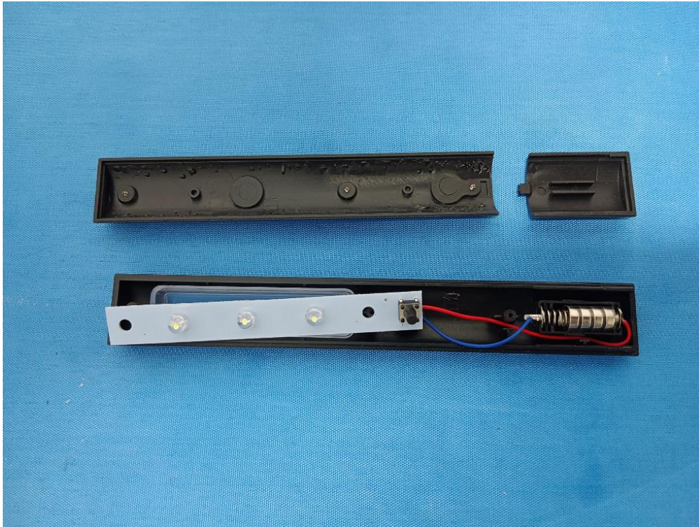
Fig.3– Internal view of the product
